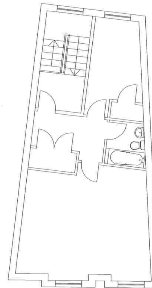
SECOND FLOOR PLAN SCALE 1:100
