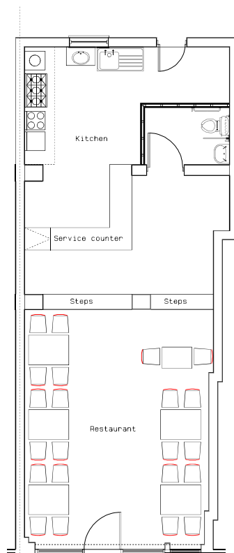
Existing ground floor 1:50
